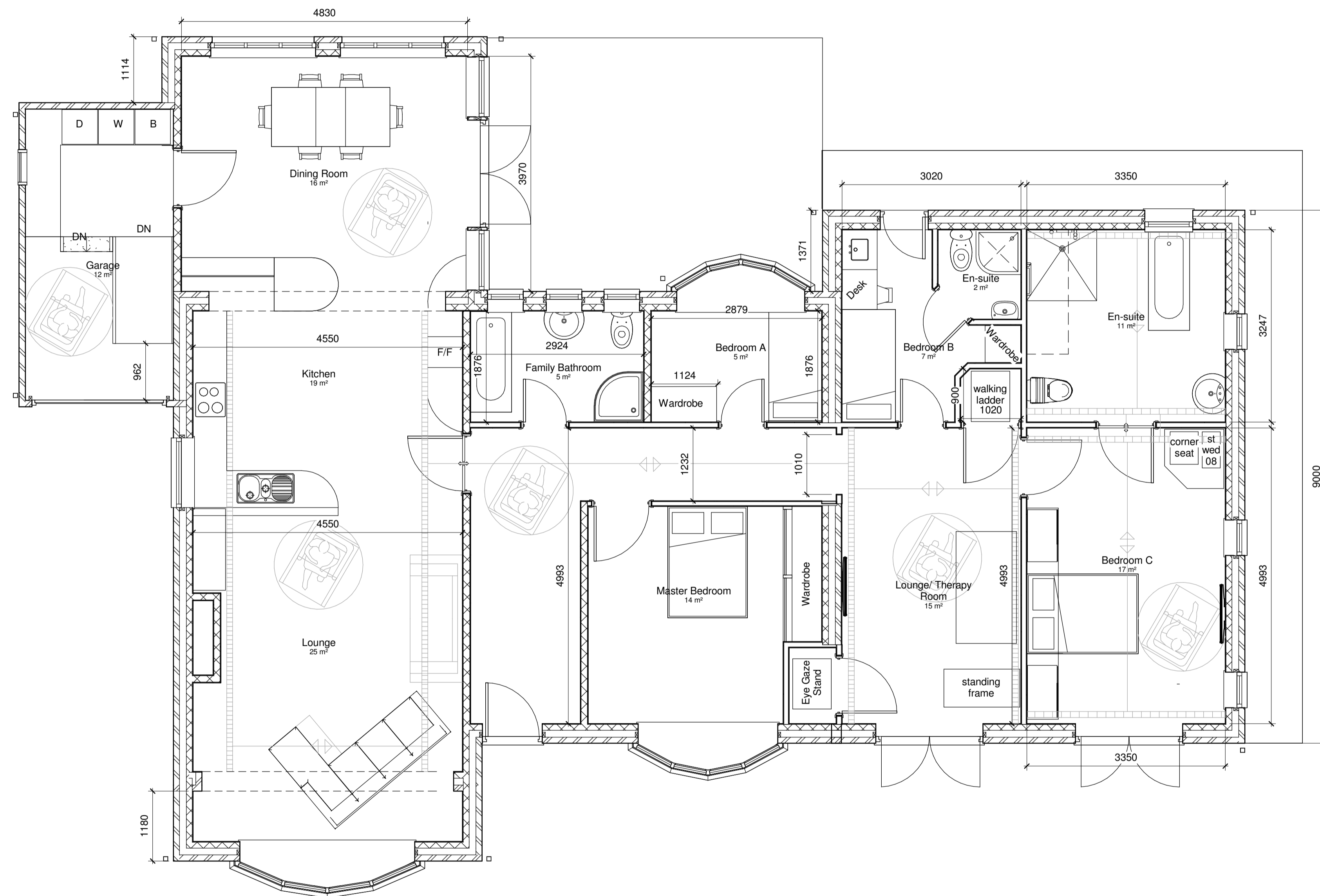
1 L0 - Ground Floor Proposed 1 : 50 @ A1
